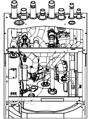
Wiring for "COMBINATION-2"
